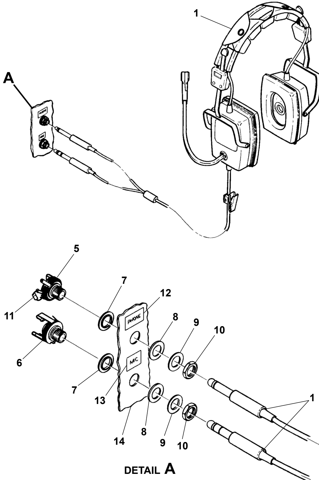
COMBINATION HEADSET AND MICROPHONE INSTALLATION Figure 01. (Sheet 1)
