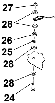
DETAIL D
