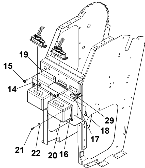
DETAIL B
