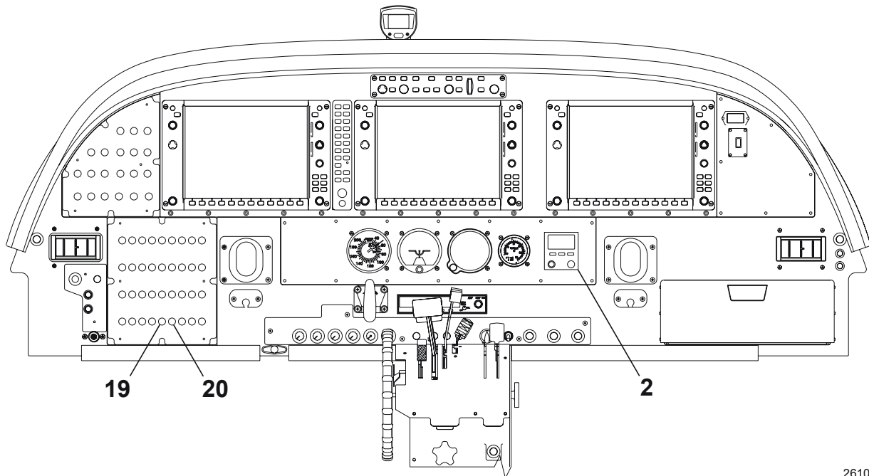
VIEW A-A KHF 1050 PANELS Figure 02. (Sheet 1)
