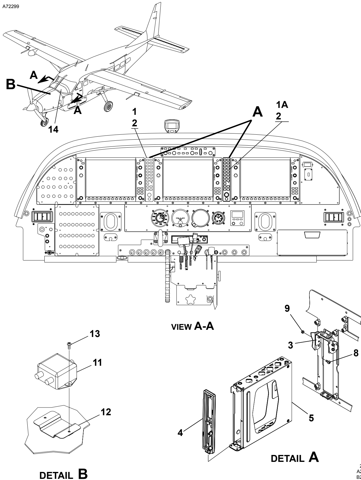
AUDIO PANEL INSTALLATION Figure 01. (Sheet 1)
