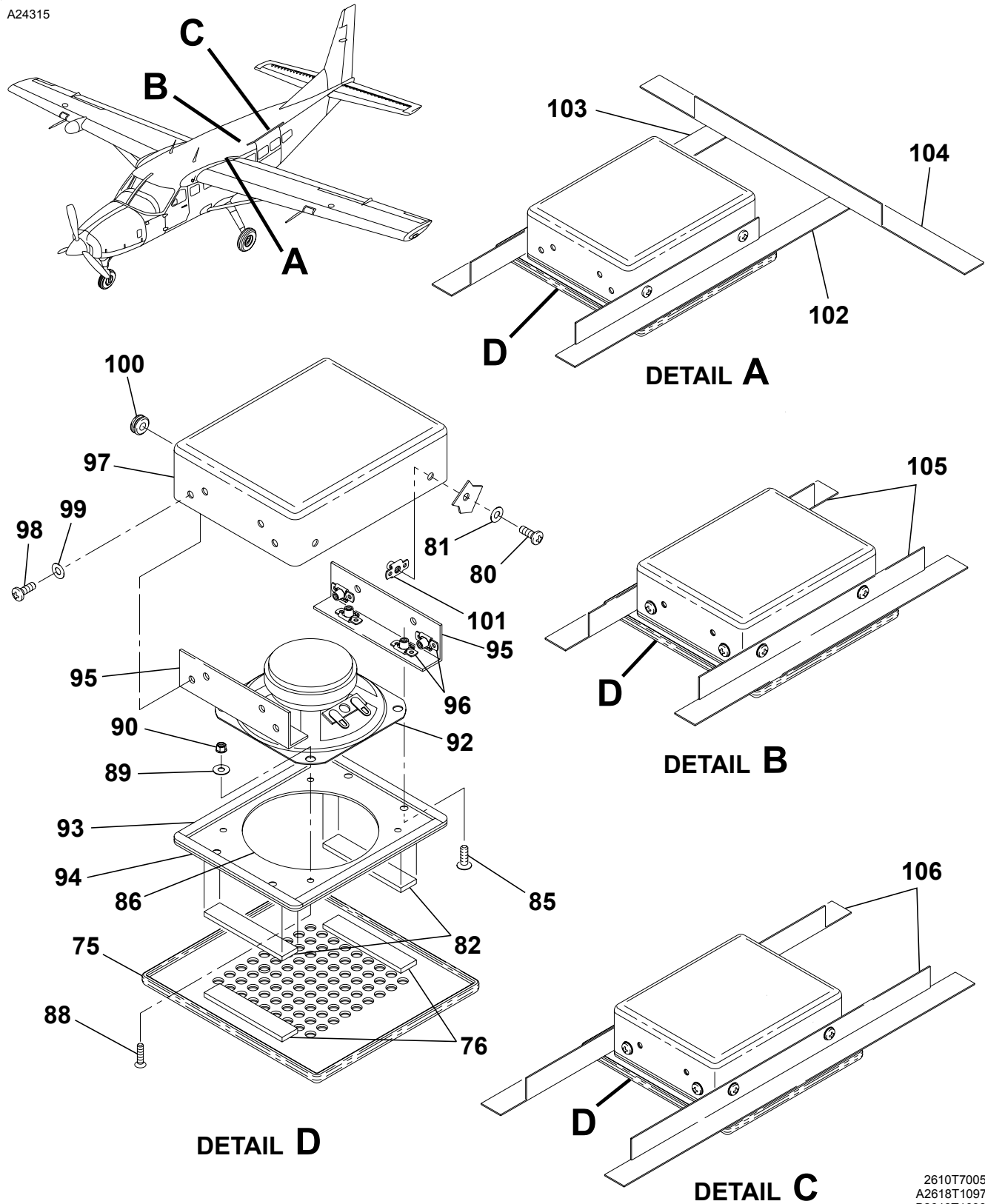
PUBLIC ADDRESS SPEAKER INSTALLATION - 208B Figure 01. (Sheet 2)
