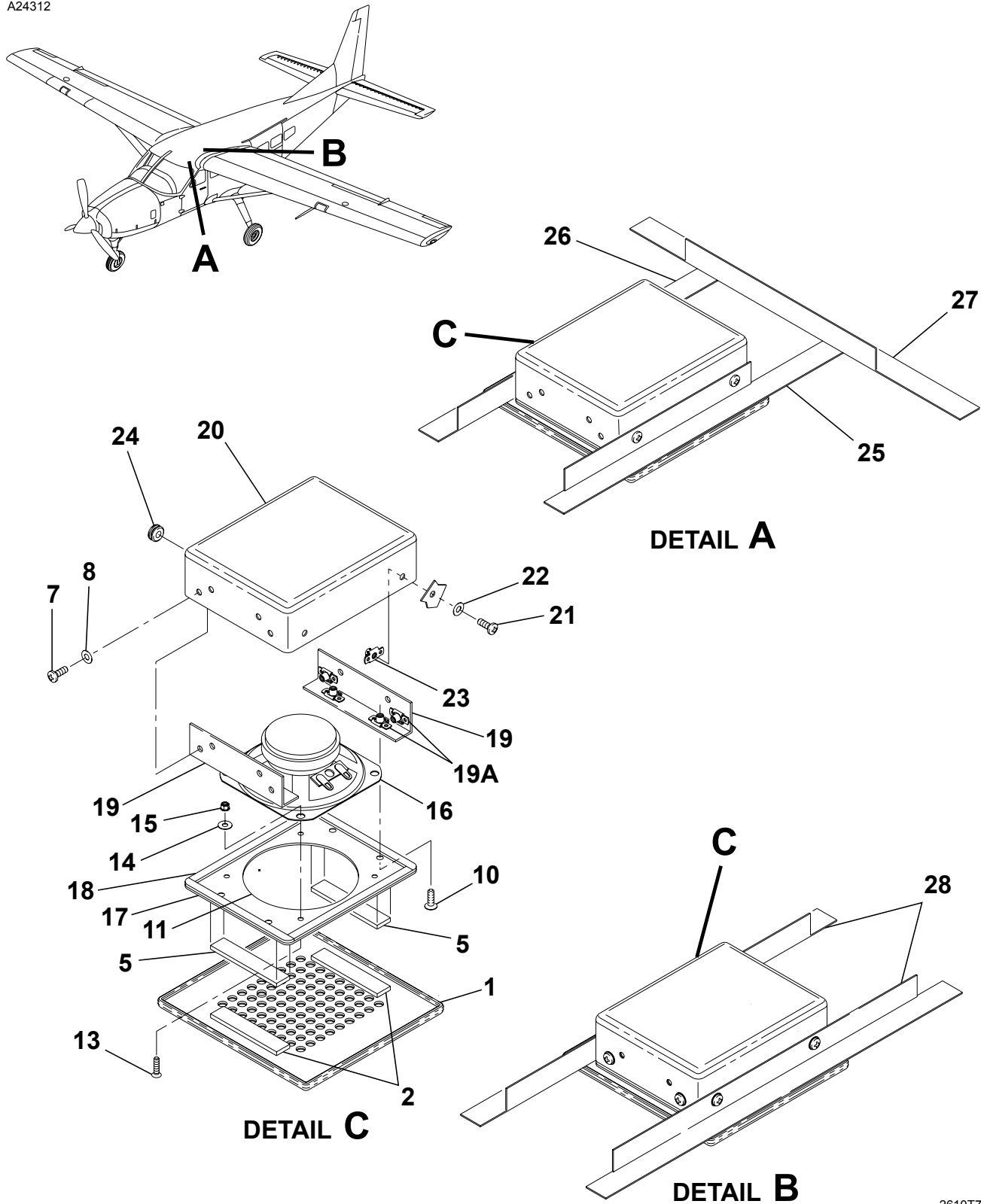
PUBLIC ADDRESS SPEAKER INSTALLATION - 208 Figure 01. (Sheet 1)
