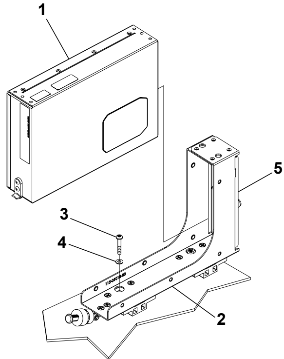
DETAIL A
