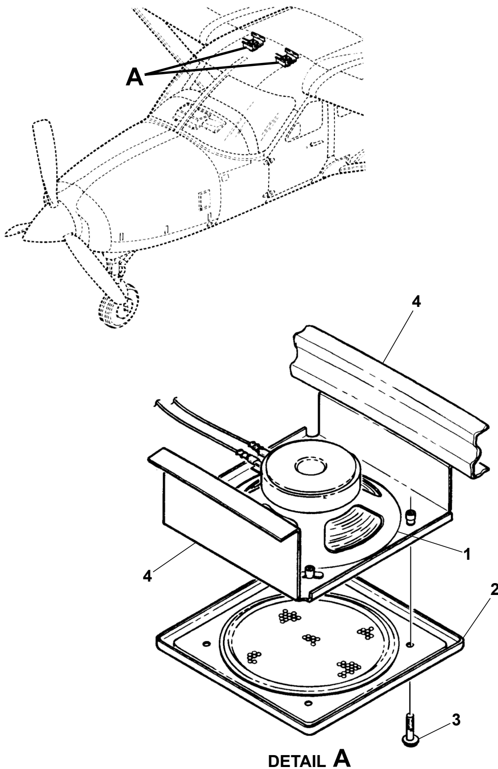
SPEAKER INSTALLATION Figure 01. (Sheet 1)
