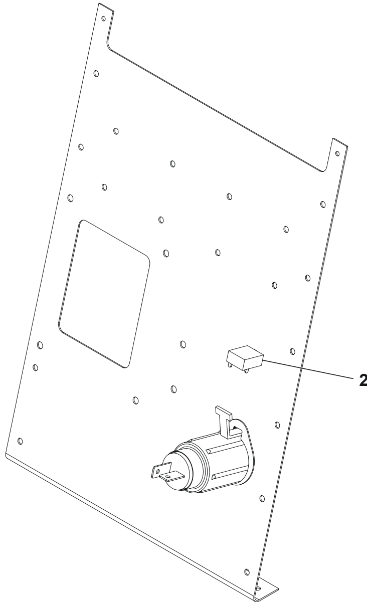
WIRING BUNDLE ASSEMBLIES - CABIN AUDIO Figure 02. (Sheet 1)
