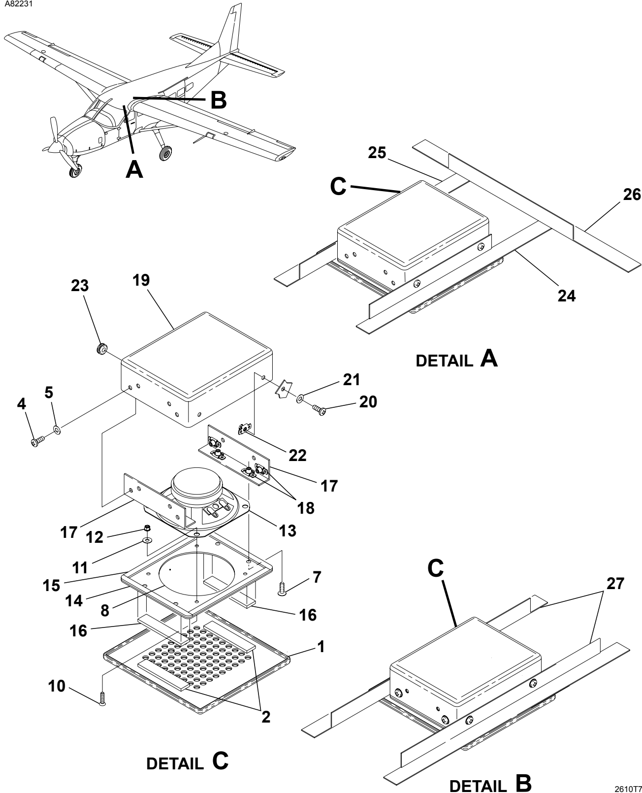
PUBLIC ADDRESS SPEAKER INSTALLATION - 208 Figure 01A. (Sheet 1)
