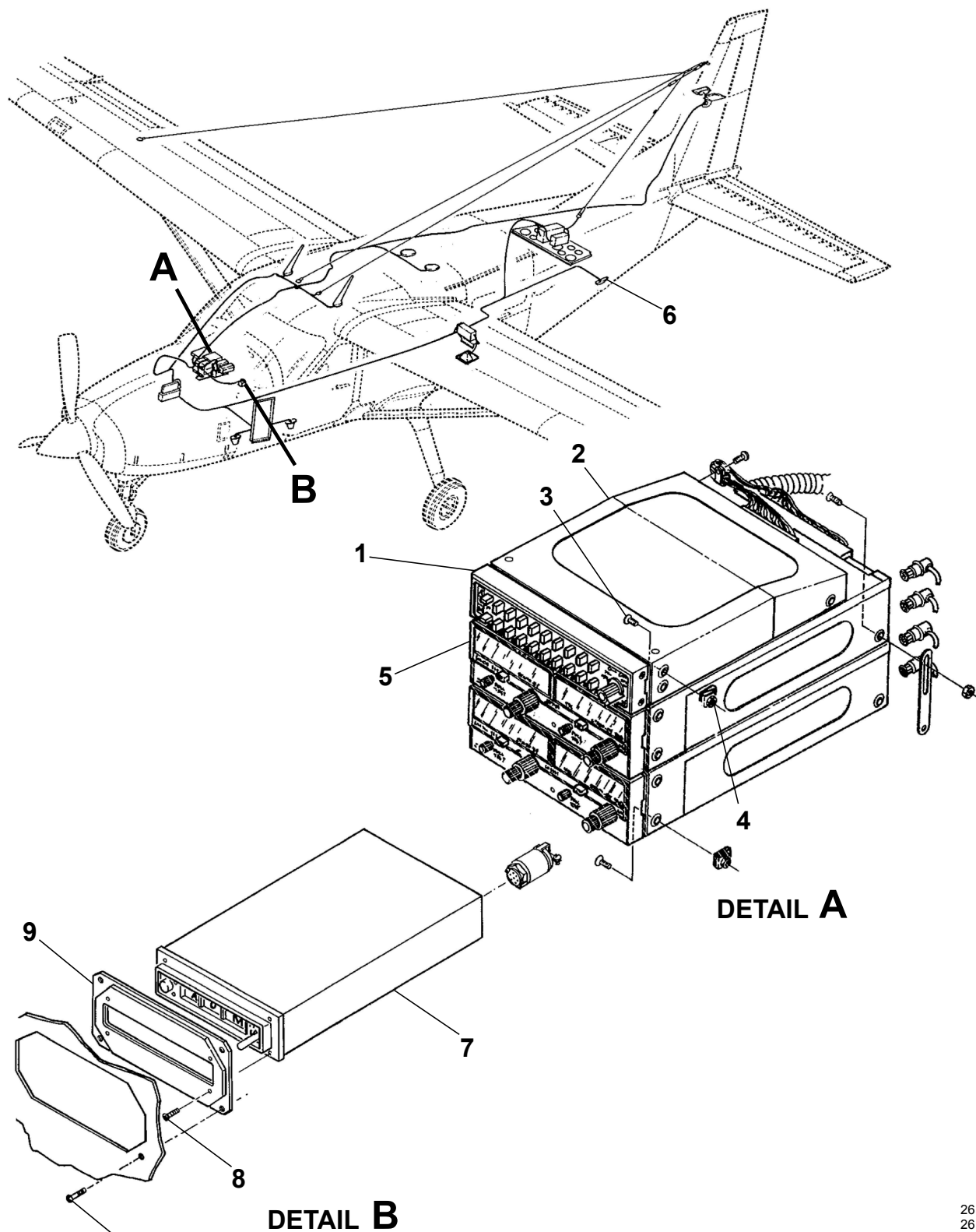
KING AUDIO INTERCOM WITH KR-21 MARKER BEACON INSTALLATION - (TYPES KMA24H-70 AUDIO PANEL AND KR-21 MARKER BEACON)
